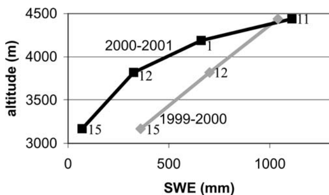
FIGURE 5. Maximum winter snow water equivalent (SWE) for Telbrung (3170 m), Sundar (3820 m), Danfedanda (4190 m), and Rambrong (4440 m) stations for winters 1999–2000 and 2000–2001. The numbers next to data points refer to station identification numbers in Table 1.
